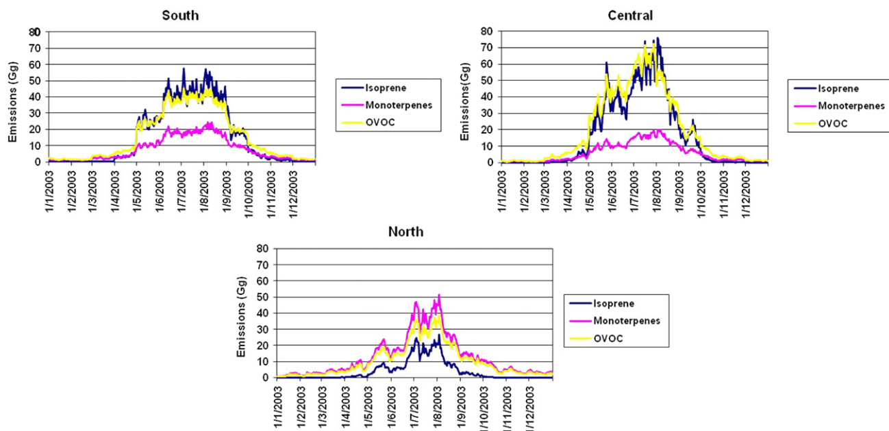
Fig. 4. Daily BNMVOC emissions (Gg) in the three spatial zones of the study area.
