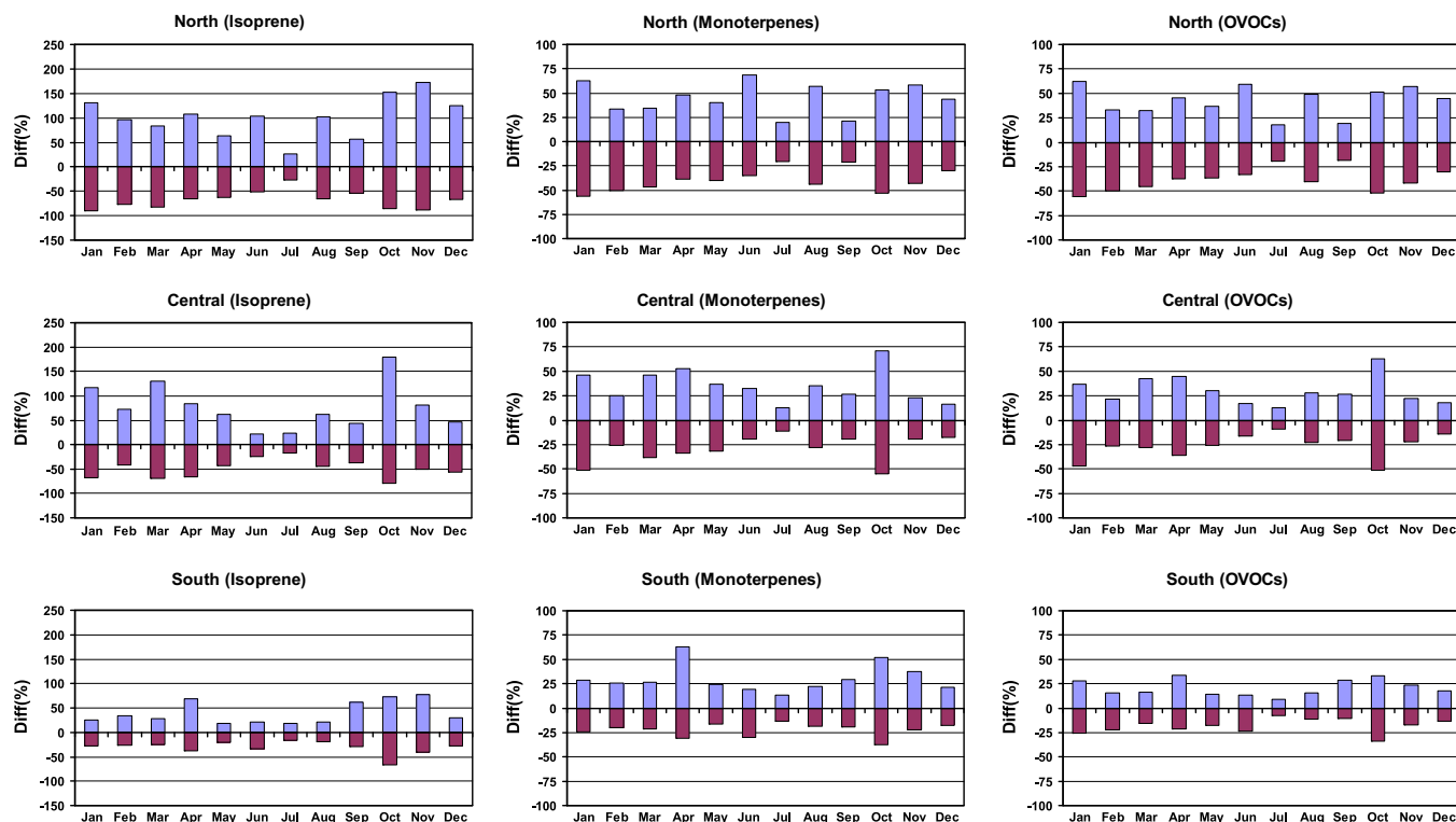
Fig. 5. Difference of the daily BNMVOC emissions from the mean monthly values in the southern, central and northern parts of the study area (reference year 2003).
